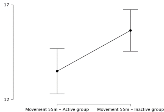
Figure 2. Descriptive plots for Movement time.
